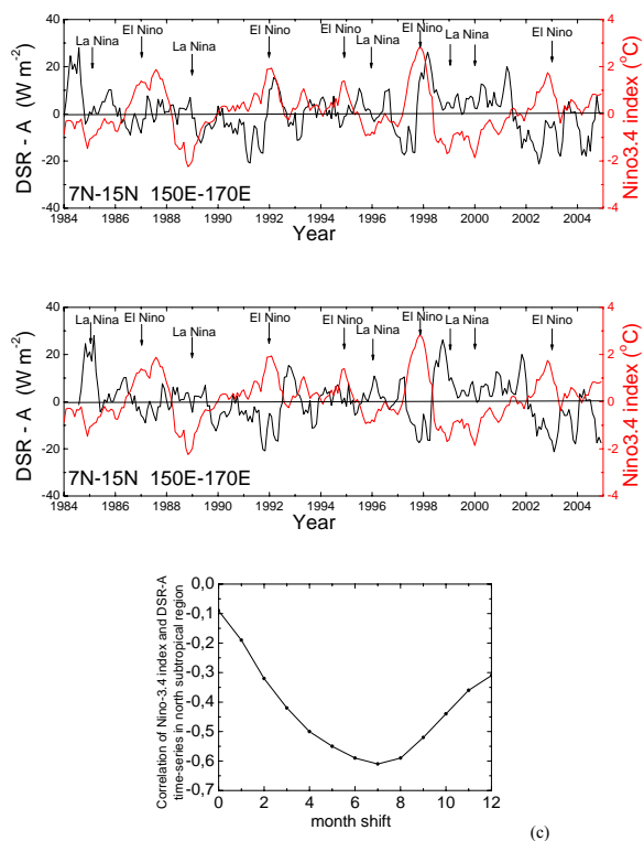
Fig. 9. (a) Time-series of downward shortwave radiation anomaly (DSR-A) at the surface (defined with respect to the average monthly DSR for the whole study period 1984–2004) in the off-equatorial western Pacific region ( 7\text{--}15^{\circ}\text{N} 150\text{--}170^{\circ}\text{E} ). Overlaid is the time-series of the Niño-3.4 index (red line). (b) The same as (a) but with the DSR-A time-series shifted by 7 months. (c) correlation coefficient of the Niño-3.4 index and the DSR-A in the 7^{\circ}\text{N} – 15^{\circ}\text{N} 150\text{--}170^{\circ}\text{E} region as a function of the number of months shift of the DSR-A.
