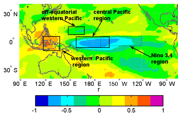
Fig. 5. Geographical distribution of correlation coefficient between DSR-A and the Niño-3.4 index.
