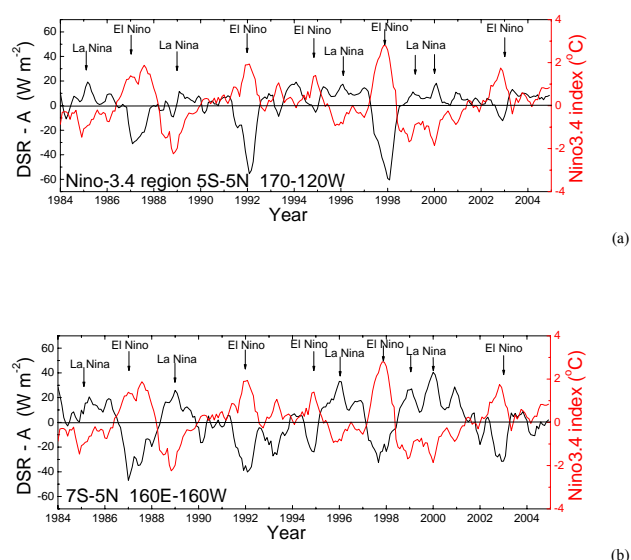
Fig. 6. Time-series of downward shortwave radiation anomaly (DSR-A) at the surface (defined with respect to the average monthly DSR for the whole study period 1984–2004) in the Niño-3.4 region (a), and in the central Pacific region ( 7^\circ \text{ S} – 5^\circ \text{ N} 160^\circ \text{ E} – 160^\circ \text{ W} ) (b). Overlaid is the time-series of the Niño-3.4 index (red line).
