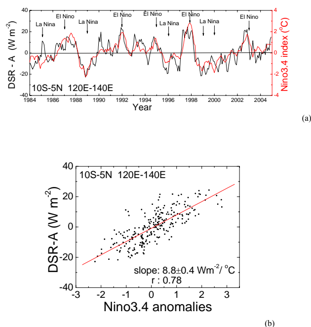
Fig. 8. (a) Time series of downward shortwave radiation anomaly (DSR-A) at the surface in the western Pacific region 10° S–5° N, 120–140° E (black line) compared with the time series of the Niño-3.4 index (red line), (b) Scatter plot between the DSR-A and the Niño-3.4 index in the western Pacific region
