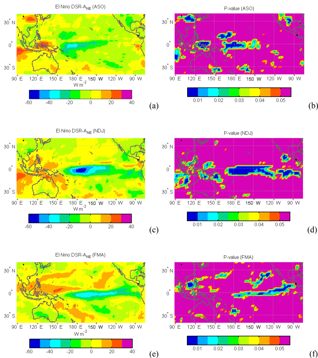
Fig. 3. Left: The distribution at 2.5 \times 2.5 spatial resolution of El Niño DSR-A NE for ASO (top panel), NDJ (middle panel), and FMA (bottom panel). Right: The distribution of P-values from a Student's t-test.
