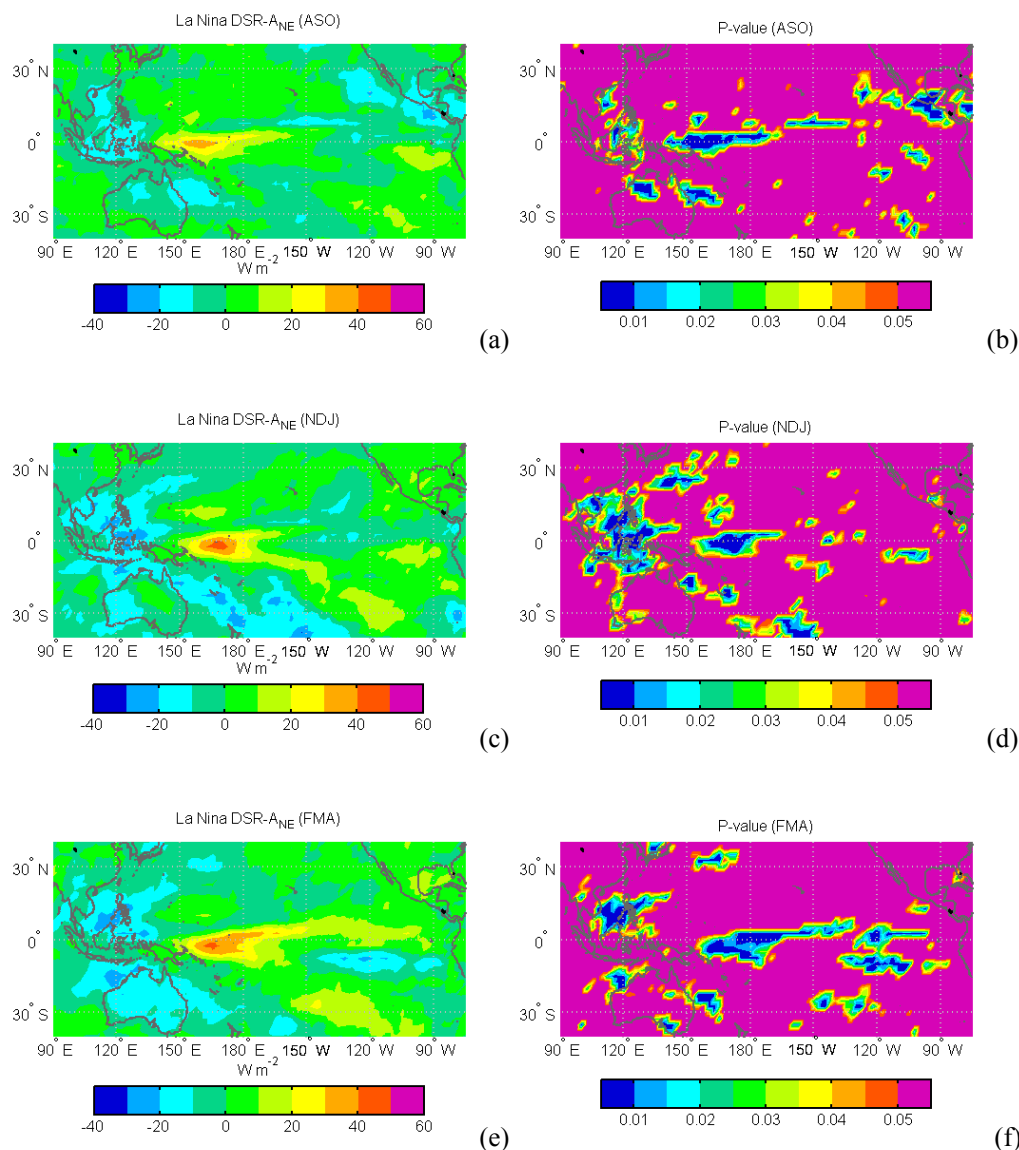
Fig. 4. Left: The distribution at 2.5 \times 2.5 spatial resolution of La Niña DSR-A_{NE} for ASO (top panel), NDJ (middle panel), and FMA (bottom panel). Right: The distribution of P-values from a Student's t -test.
