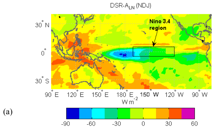
Fig. 2. Differences in the mean downward shortwave radiation at the surface (DSR), between the El Niño and La Niña years, over the tropical and subtropical Pacific for the period of November, December and January (NDJ).
