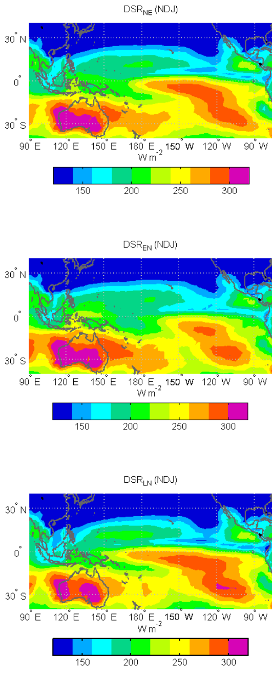
Fig. 1. The distribution of downward shortwave radiation at the surface (DSR), over the tropical and subtropical Pacific for the three month period November, December, January (NDJ); (a) eleven neutral years average, (b) average for five El Niño years, (c) average for five La Niña years.
