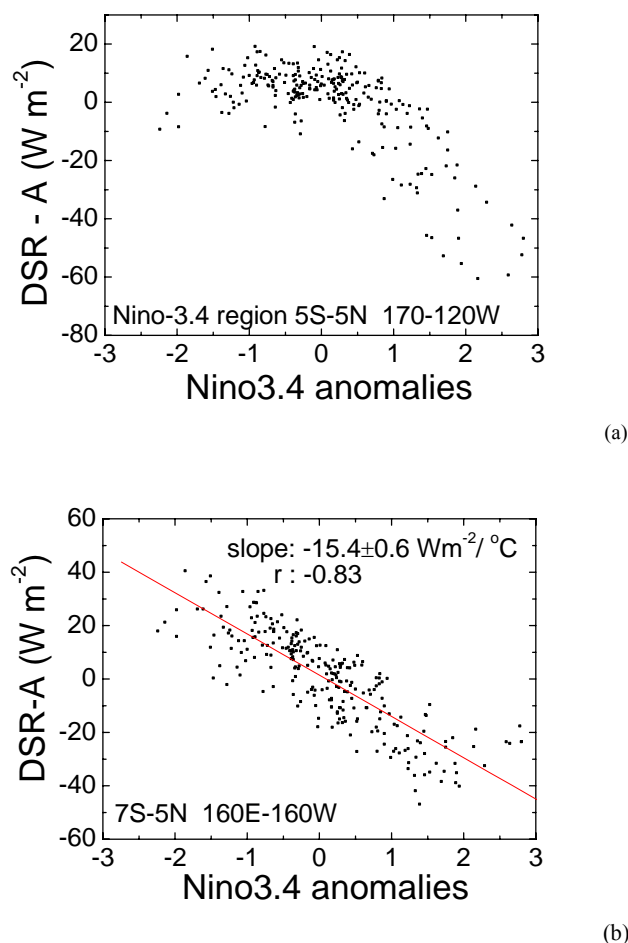
Fig. 7. Scatter plot between the Niño-3.4 index and the DSR-A in the: (a) Niño-3.4 region and (b) the central Pacific region (7° S–5° N 160° E–160° W).
