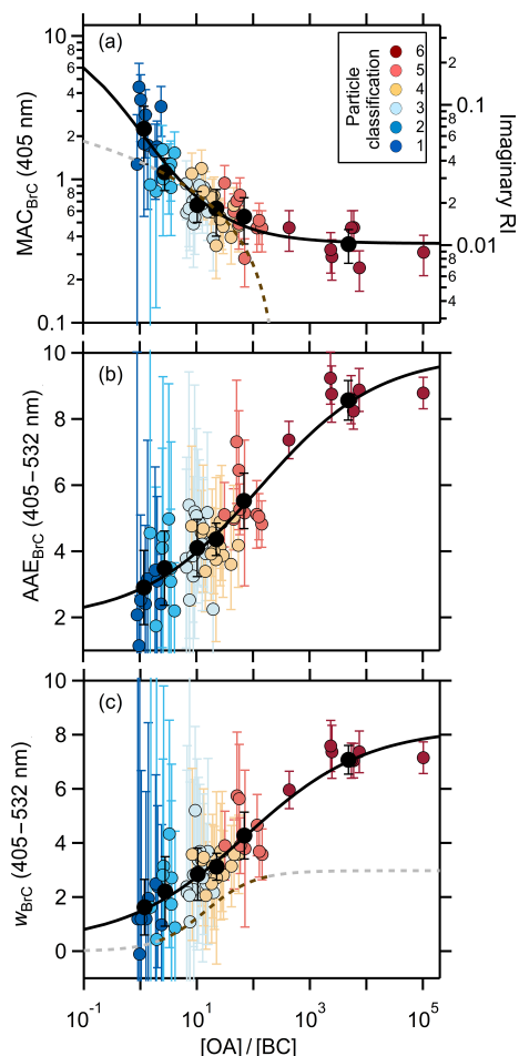
Figure 5. Relationship between (a) MAC_{BrC,405\text{ nm}} , (b) AAE_{BrC,405-532} , and (c) w_{BrC,405-532} and the [OA]/[BC] mass ratio. The solid lines are sigmoidal fits to the observations against \log([OA]/[BC]) . The dashed lines are based on the parameterization of Saleh et al. (2014), with the brown color indicating the measuring range in that study and the gray color extrapolated. Results for individual burns are shown as points colored by the particle class, and class average values are shown as black circles. Uncertainties on the class averages are 1\sigma based on measurement variability. Uncertainties for the individual burns are determined from error propagation.
