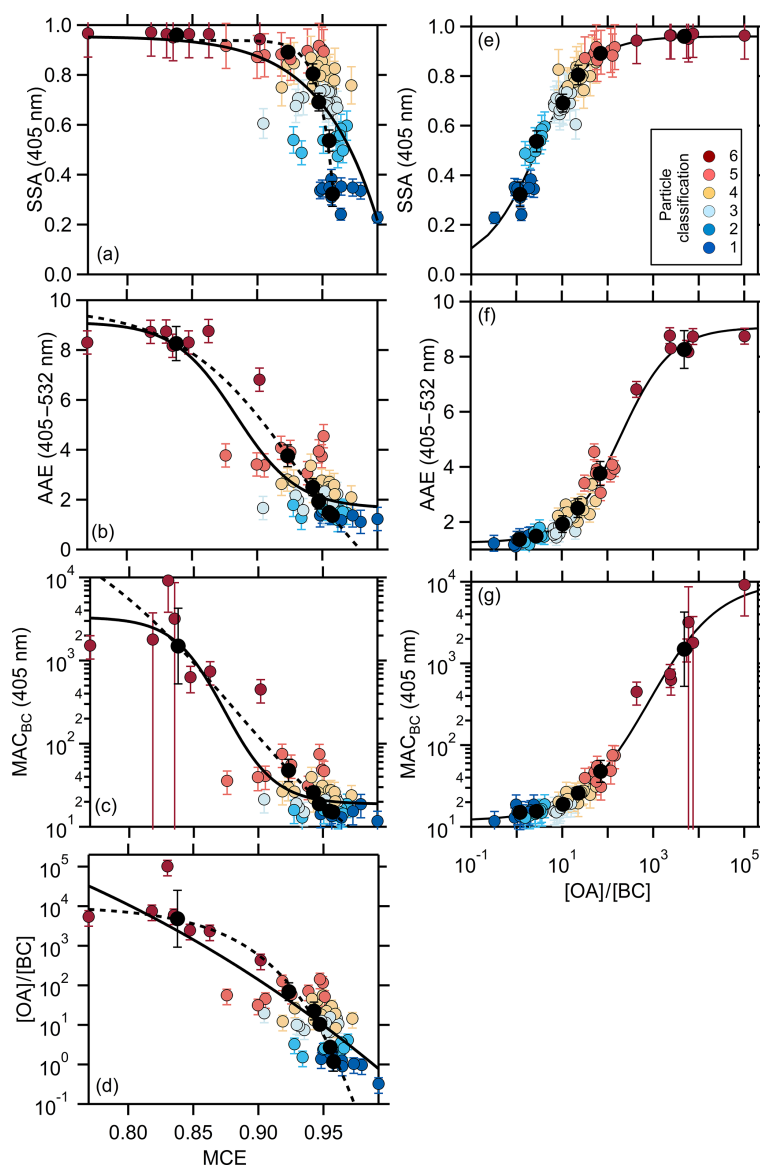
Figure 1. (a–d) Relationship between (a) the SSA_{405\text{ nm}} , (b) the AAE_{405-532} , (c) the MAC_{BC} , and (d) the [OA]/[BC] mass ratio and the modified combustion efficiency, MCE. Results for individual burns are shown as points colored by the particle class, and class average values are shown as black circles. Uncertainties on the class averages are 1\sigma based on measurement variability and uncertainties for the individual burns are from error propagation of measurement uncertainties. The solid black lines are fits to the individual burns (colored points) while the dashed black lines are fits to the class averages (Table S2). (e–g) Relationship between (e) the SSA_{405\text{ nm}} , (f) the AAE_{405-532} , and (g) the MAC_{BC} on the [OA]/[BC] mass ratio. The solid black lines here are sigmoidal fits to the individual burns. Fits to the class averages are similar.
