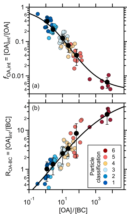
Figure 3. Relationship between the total [OA] / [BC] mass ratio and (a) the fraction of OA that is internally mixed with BC, f_{OA,int} ; and (b) the OA-to-BC mass ratio for only the internally mixed OA. Results for individual burns are shown as points colored by the particle class, and class average values are shown as black circles. Uncertainties on the class averages are 1\sigma based on measurement variability. Black lines are sigmoidal fits to the data, in log–log space.
