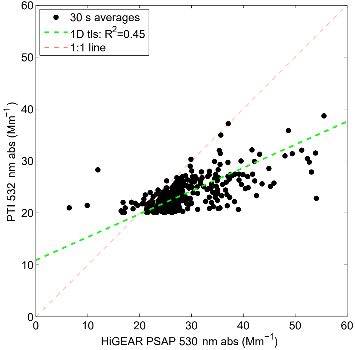
30 s average data, PTI vs PSAP absorption, ORACLES-2016
