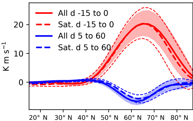
(c) \Delta v'T' 100 hPa
