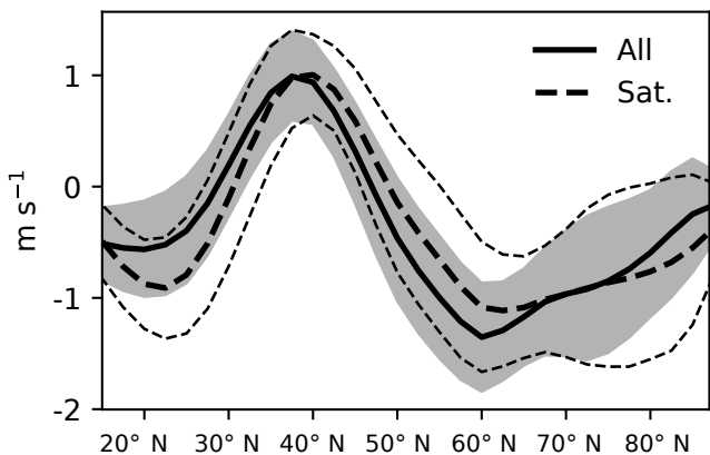
(a) \Delta [u] d 5 to 60
