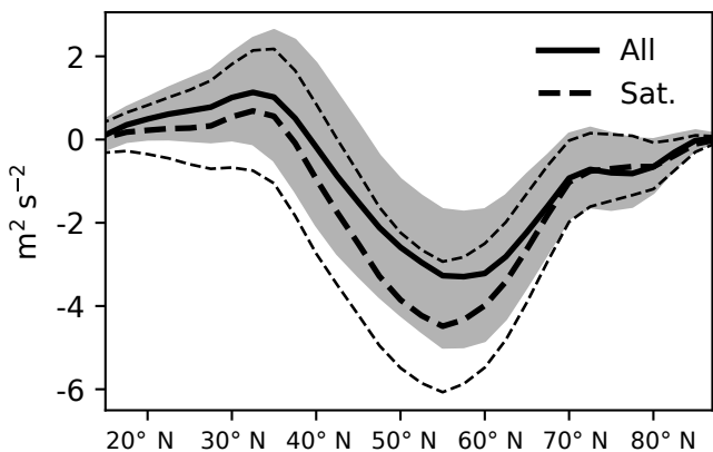
(b) \Delta [u'v'] d 5 to 60
