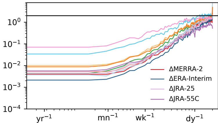
(c) u 500 hPa, 40° N 1979 to 2010
