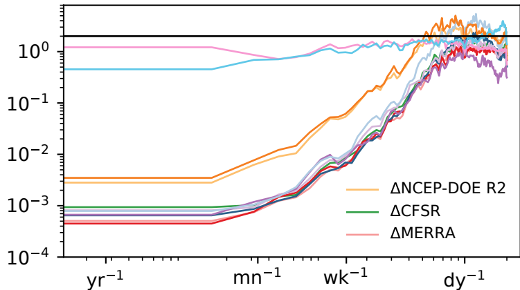
(c) u 500 hPa, 40° N 1979 to 2010
