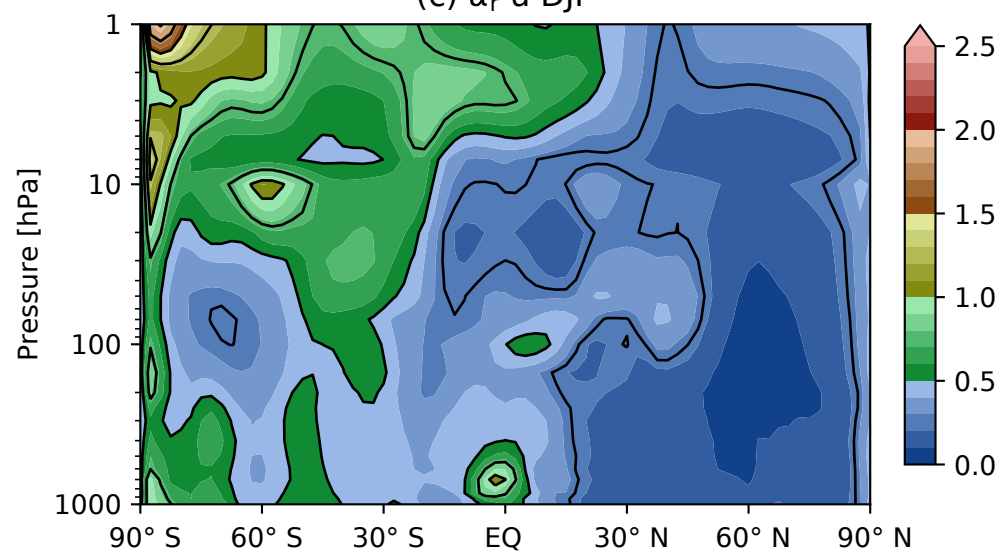
(e) \delta u DJF
