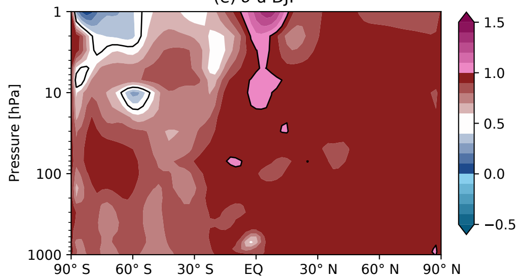
(e) \delta u DJF
