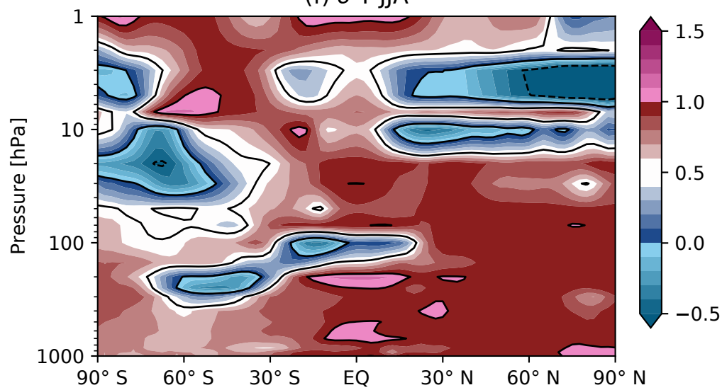
(f) \delta T JJA
