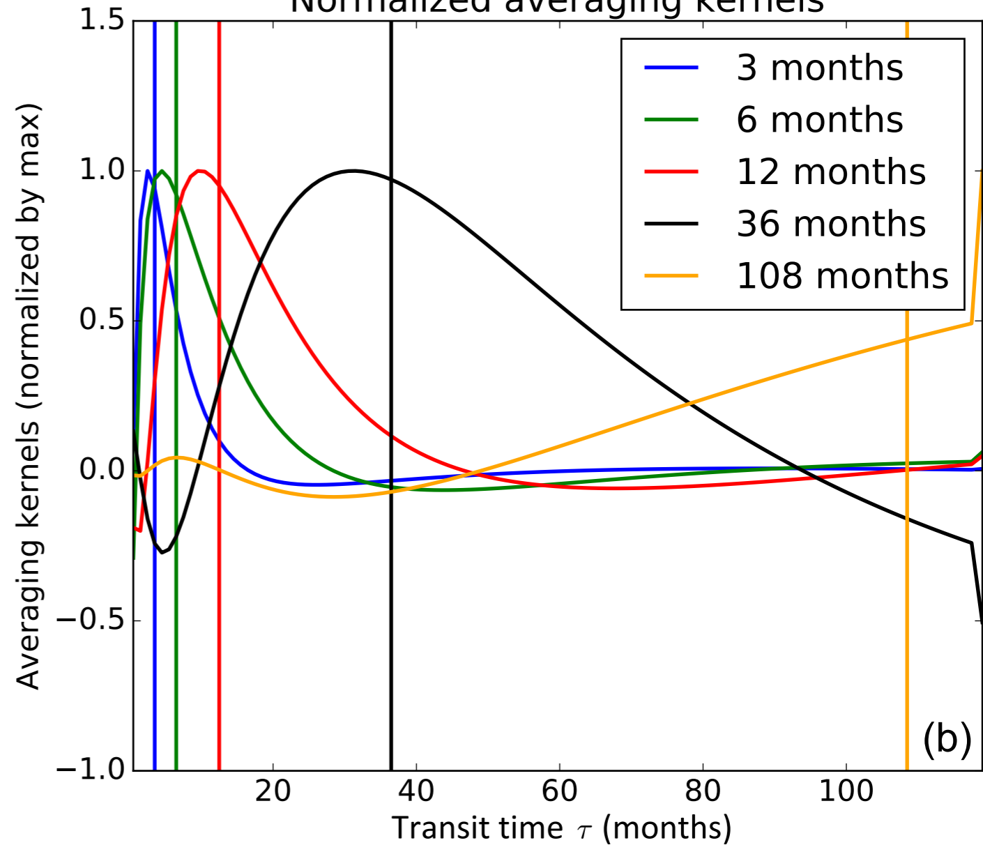
Normalized averaging kernels
