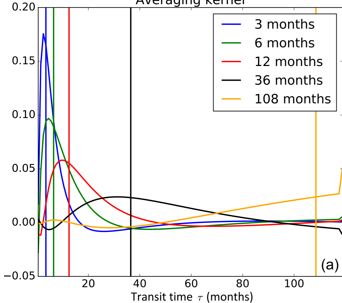
Averaging kernel
