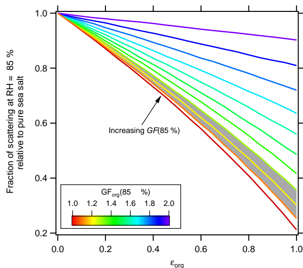
Figure 6. Calculated fraction of scattering relative to pure sea salt particles at 85 % RH as a function of \epsilon_{org} , assuming the OM component of the SSA particles have the same constant hygroscopicity and a refractive index of 1.55 and the SSA particles follow the ZSR mixing rules. The different curves are colored according to the assumed GF_{org}(85\%) value, ranging from 1.0 to 2.0, given GF_{sea\ salt}(85\%) = 2.1 . The gray band shows the range of GF_{org} values indicated by the current measurements.
