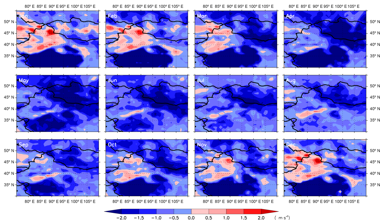
Figure 8. Annual cycle of the near-surface wind speed difference at 06:00 UTC between NLLJ and non-NLLJ days.
