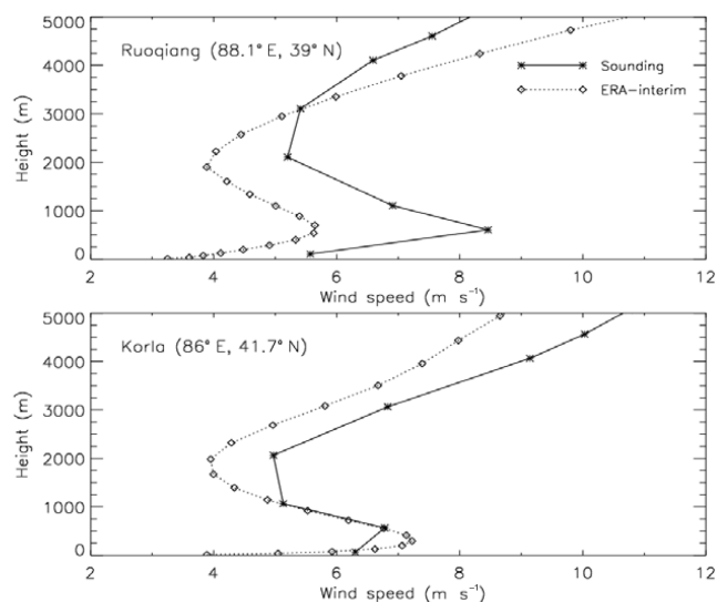
Figure 4. Mean wind speed profiles at 00:00 UTC based on radiosondes (solid line) and ERA-Interim (dotted line) at (a) Ruoqiang and (b) Korla sites for 2000–2012.
