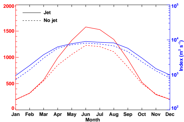
Figure 9. Monthly averaged convection boundary layer height at 06:00 UTC, and momentum index at 00:00 UTC over the TD.
