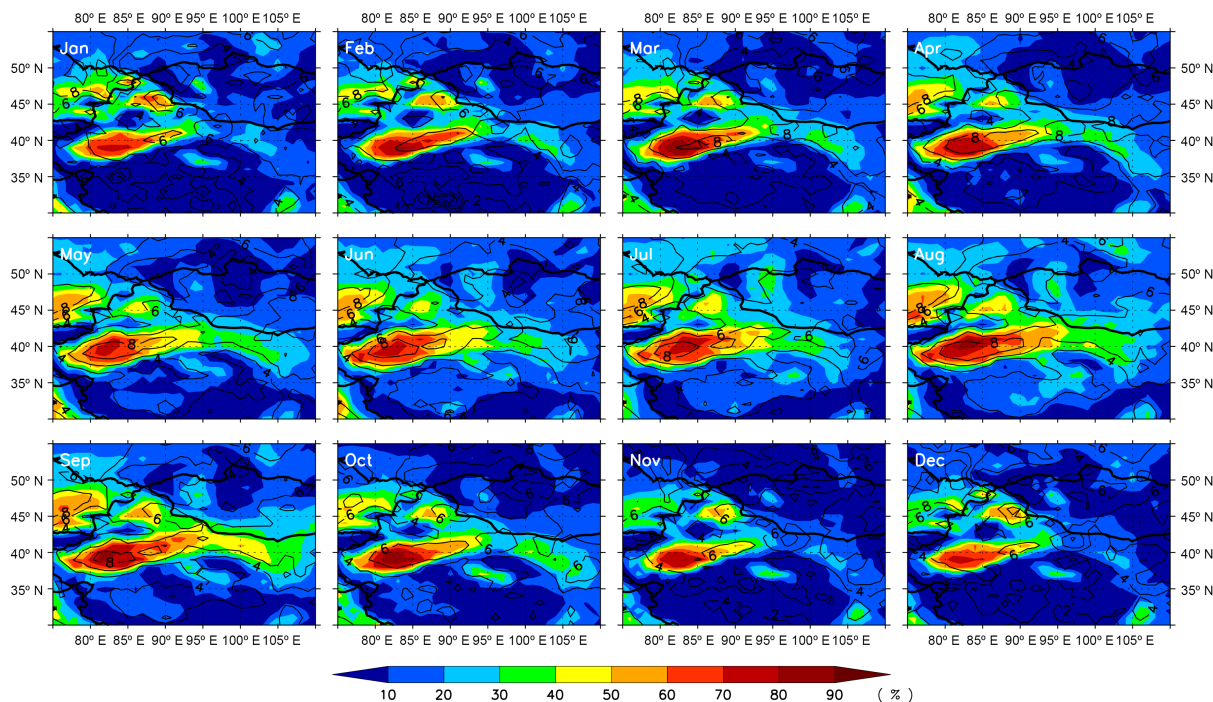
Figure 5. Monthly mean occurrence of NLLJs (colors) with jet core wind speed (contours) at 00:00 UTC by applying the NLLJ detection algorithm to the ERA-Interim reanalysis data for 2000–2013.
