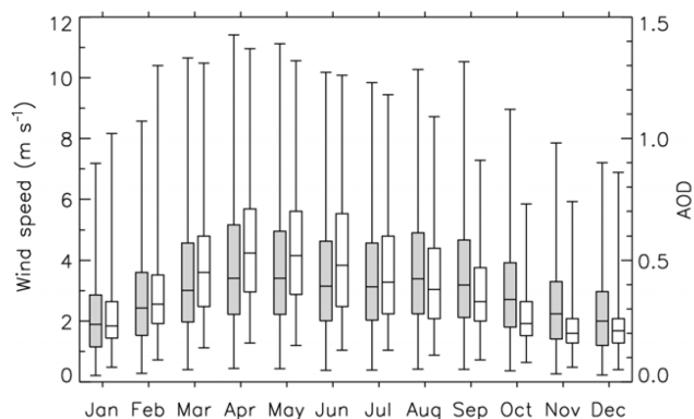
Figure 2. Annual cycles of wind speed (gray bars) and AOD (white bars) from 2000 through 2013 over the Taklimakan Desert. The horizontal line through each box represents that monthly median value; the top and bottom of the boxes mark 75th and 25th percentiles, respectively; and whiskers mark the 95th and 5th percentiles.
