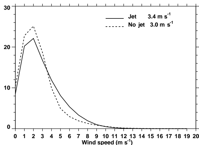
Figure 7. Frequency distribution of 10 m wind speed at 06:00 UTC (i.e., roughly at 11:30 LT) over the Taklimakan.
