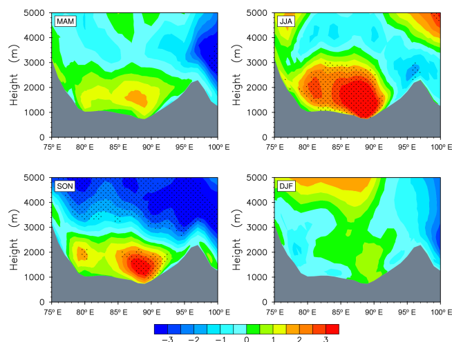
Figure 10. Seasonal longitudinal cross sections of daily wind composite difference between high and low AOD days along 40^{\circ} N. Stippled areas are significant at the 95 % level. Gray areas represent terrain.
