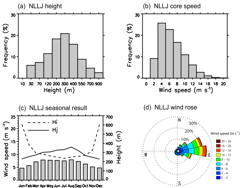
Figure 6. Climatological features of NLLJ over the Tarim Basin (38–42° N, 78–88° E). (a) Frequency distribution of NLLJ height. (b) Frequency distribution of NLLJ speed. (c) Monthly mean jet core speed (gray bars), NLLJ core height (solid line), and inversion height (dashed line). (d) Jet core wind direction and speed distribution at 00:00 UTC (i.e., 05:30 LT) from ERA-Interim reanalysis from 2000 through 2013.
