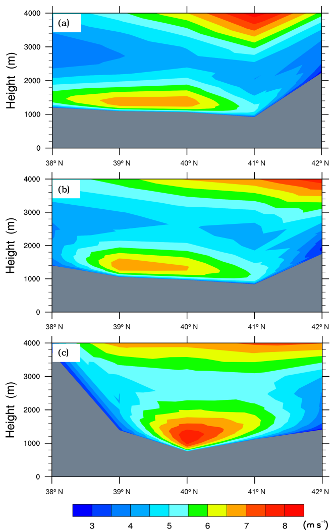
Figure 3. Latitude–height cross sections of annual mean wind speed at three longitudes of (a) 82° E, (b) 85° E, and (c) 88° E from ERA-Interim reanalysis averaged over 2000–2013. Gray areas represent the terrain elevation.
