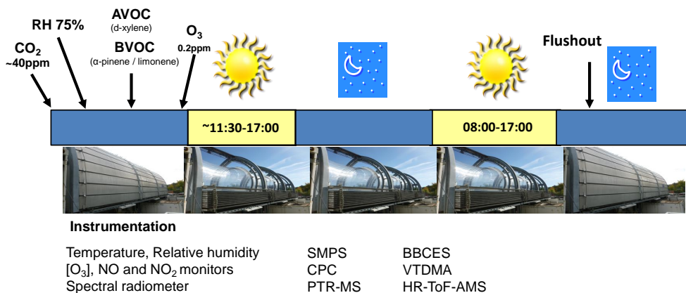
Figure 1. Schematic of the experimental procedure and instrumentation used for measuring the evolution of secondary organic aerosol over a diurnal cycle. All experiments began around 11:30 local time. Acronyms: SMPS – scanning mobility particle sizer; CPC – condensation particle counter; PTR-MS – proton transfer reaction mass spectrometer; BBCES – broadband cavity-enhanced spectrometer; VTDMA – volatility tandem differential mobility analyzer; HR-ToF-AMS – high-resolution time-of-flight aerosol mass spectrometer.
