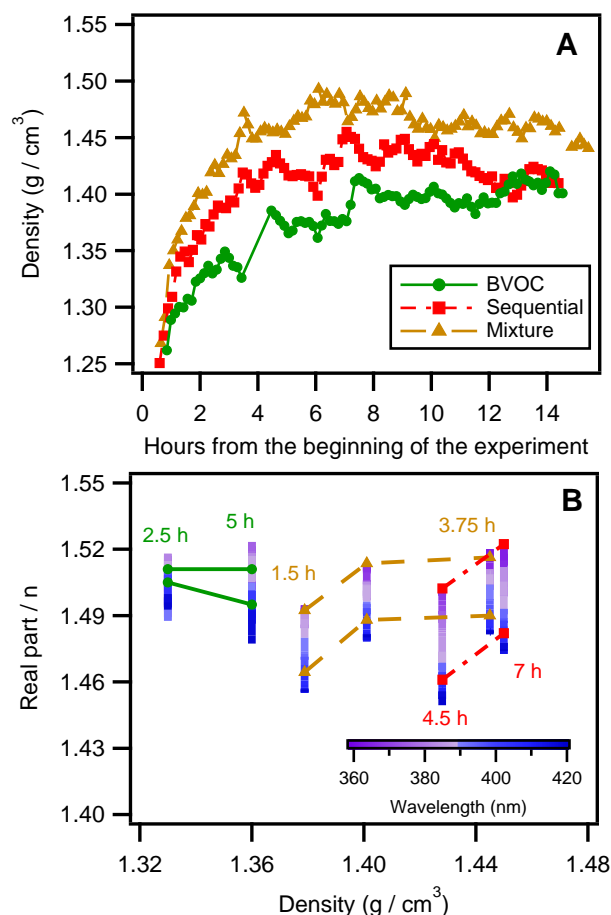
Figure 6. (A) Time series of the density measured for the BVOC (green circles), the sequential (red squares), and the mixture (orange triangles) experiment. (B) The change in time of the real part of the RI vs. density for each experiment performed. The color bars show the span in the RI for the wavelengths measured; the time span between the measurements is written above (for the BVOC and sequential experiments) and below (the mixture experiment) each set of measurements.
