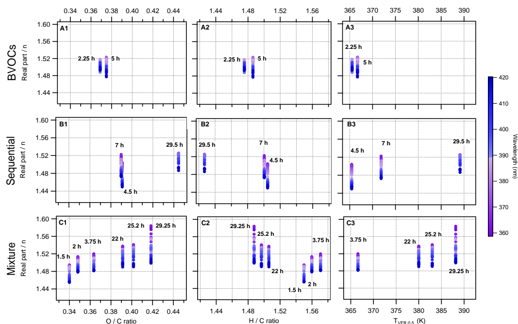
Figure 4. The change in time (given in hours, shown next to the retrieved values) for the retrieved real part of the RI as a function of O/C ratio (panels A1, B1, and C1), H/C ratio (panels A2, B2, and C2), and T_{VFR0.5} (the temperature at which the volume fraction remaining was reduced by half; panels A3, B3, and C3). The top panels – (A1), (A2) and (A3) – show the results for the SOA produced from a 1 : 1 mixture of \alpha -pinene and limonene. The middle panels – (B1), (B2), and (B3) – show the results for the SOA produced from the mixture of \alpha -pinene, limonene, and p -xylene- d_{10} . The lower panels – (C1), (C2), and (C3) – show the results for the SOA produced from the sequential addition of the mixture of \alpha -pinene and limonene followed by p -xylene- d_{10} . The color scale indicates the measured wavelength. For clarity, the error bars for the O/C (31 %), H/C (10 %), and T_{VFR0.5} are not shown. The average error for the T_{VFR0.5} is 2.3 K.
