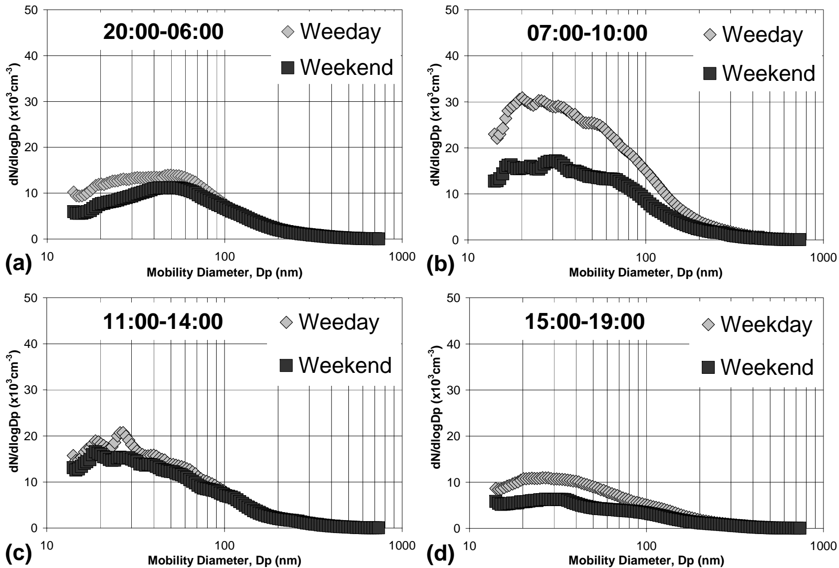
Figure S1. Diurnal patterns in average particle number size distributions on weekdays and weekends at site W2 in August.
