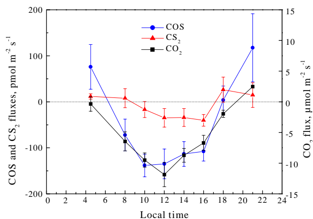
Fig. 5. Average diurnal variation in the COS, CS 2 and CO 2 fluxes. The error bars indicate standard errors of the mean.
