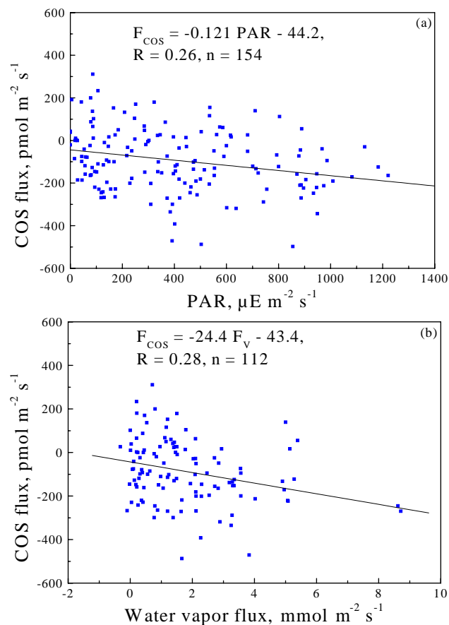
Fig. 6. Correlation of the COS flux to (a) photosynthetically active radiation (PAR) and (b) the H 2 O flux ( F_v ).
