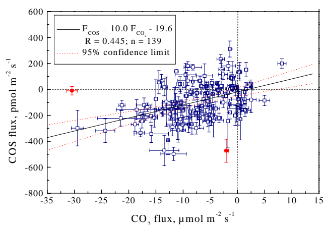
Fig. 7. Correlation between the COS and CO 2 fluxes. The vertical and horizontal bars present the estimated errors of the observed COS and CO 2 fluxes. The two outliers marked with filled circles were not included in the regression since the results are too sensitive to them.
