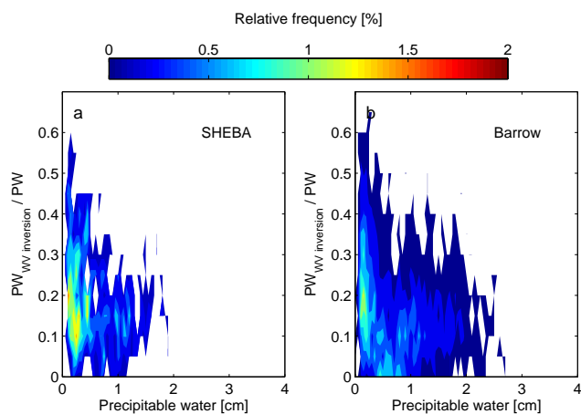
Fig. 11. The RFDs of maximum WV inversion structure PW_{\text{WV Inversion}} normalized by the total column PW as a function total column PW (in cm) for (a) SHEBA (b) Barrow radiosounding profiles.
