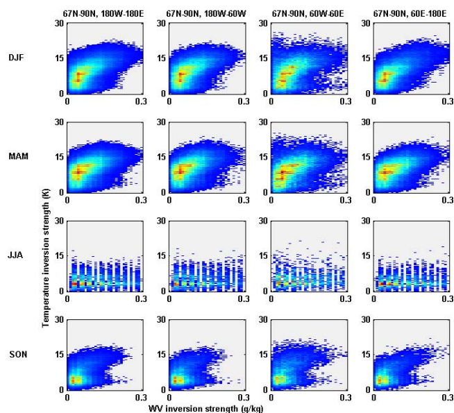
Fig. 7. The joint histograms of temperature and WV inversion strengths for different seasons and for the entire Arctic (left-most column) and for three distinct regions ( 180^{\circ} W– 60^{\circ} W, 60^{\circ} W– 60^{\circ} E, and 60^{\circ} E– 180^{\circ} E).
