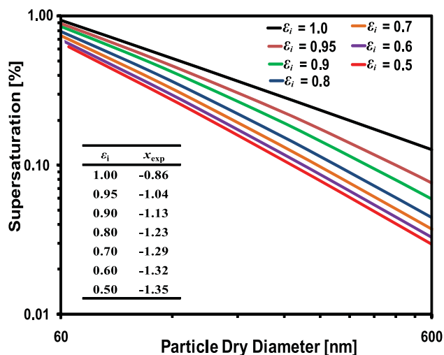
Fig. 8. s_c - D_{\text{dry}} lines for different values of \varepsilon_i computed at \sigma_w = 0.072 \text{ N m}^{-1} , T = 298.15 \text{ K} , A_{\text{FHH}} = 2.25 , B_{\text{FHH}} = 1.20 , \kappa = 0.10 . The inset table shows theoretical exponent associated with s_c - D_{\text{dry}} lines shown in the main figure.
