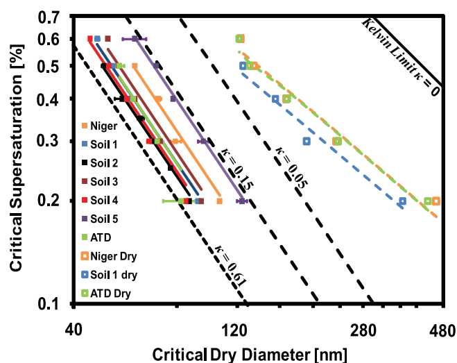
Fig. 2. CCN activation curves for different dust types considered in this study. Solid symbols refer to wet generated CCN activity and solid lines show \kappa -KT fits. Open symbols refer to dry generated CCN activity and dashed lines are FHH adsorption activation fits (Data obtained from Kumar et al., 2011). Also shown in black dashed lines are \kappa -KT lines.
