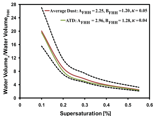
Fig. 7. Ratio of water volume required by KT over FHH-AT to activate CCN as a function of supersaturation. Simulations are performed with values of adsorption ( A_{\text{FHH}} , B_{\text{FHH}} ) and \kappa for average dust aerosol. Dashed lines represent simulation representing upper and lower limit of dust relevant adsorption parameters.
