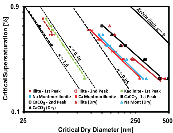
Fig. 4. CCN activation curves for different mineral and clays types considered in this study. Solid and open square (■, □) symbols refer to wet generated CCN activity and dashed lines show \kappa -KT fits. Open triangle ( \Delta ) refers to dry generated CCN activity and solid lines are FHH adsorption activation fits (obtained from Kumar et al., 2011).
