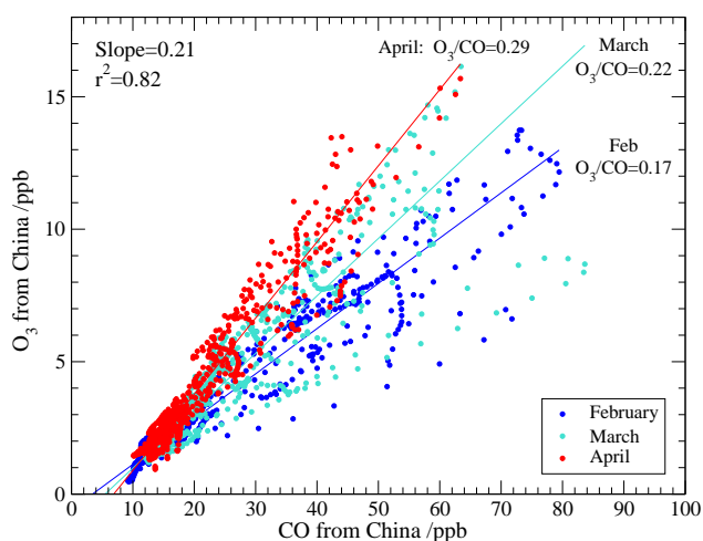
Fig. 8. Relationship between Chinese contributions to surface O_3 and CO over Tokyo revealing the increase in photochemical activity between February and April in 2001.
