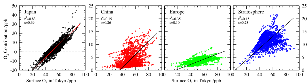
Fig. 9. Contributions of Japanese, Chinese and European industrial sources and transport from the stratosphere to hourly surface O 3 over Tokyo as a function of total modelled surface O 3 . Graphs are labelled with the correlation coefficient ( r ) and slope ( s ).
