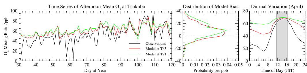
Fig. 3. Comparison of afternoon-mean O_3 observations (12:00–16:00 h JST) at Tsukuba WMO/GAW station (black) with CTM results at T21 (green) and T63 (red) resolution. Right-hand panels show the distribution of the hourly model bias and the monthly mean diurnal variation in observed and modelled O_3 in April.
