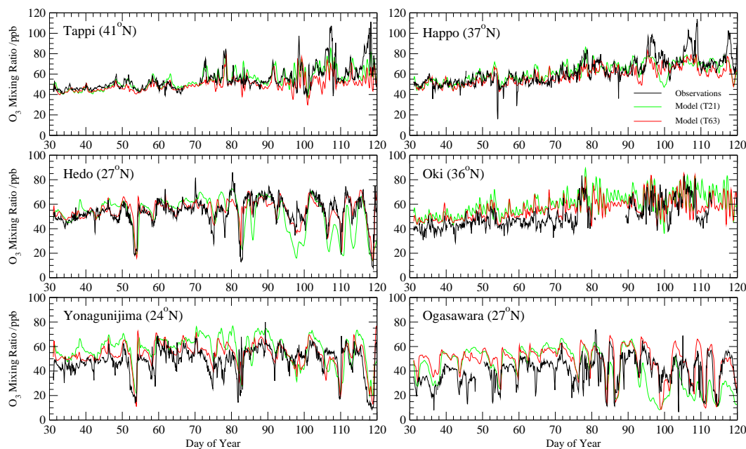
Fig. 4. Time series of hourly-mean O_3 observations at selected remote EANET and WMO/GAW measurement sites in February–April 2001 (black) and FRSGC/UCI CTM results at T21 (green) and T63 (red) resolution.
