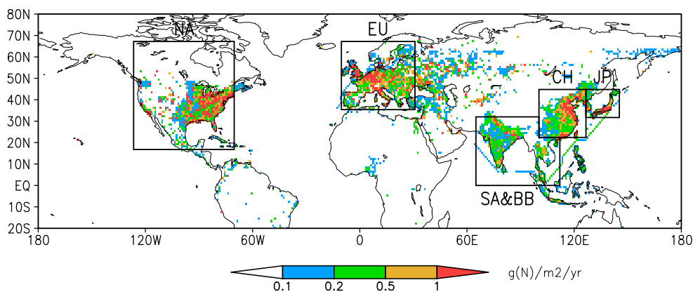
Fig. 5. Distribution of anthropogenic surface \text{NO}_x emissions ( \text{g N m}^{-2} \text{yr}^{-1} ) used in this study (Olivier et al., 1996; Streets et al., 2003) showing the principal source regions considered here.
