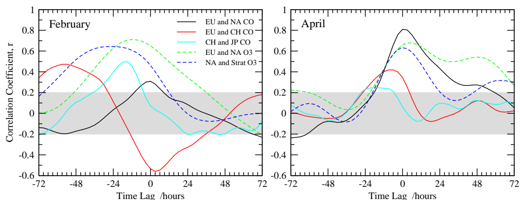
Fig. 10. Correlation between the contributions of key source regions to O 3 and CO over Tokyo in February (left) and April (right).
