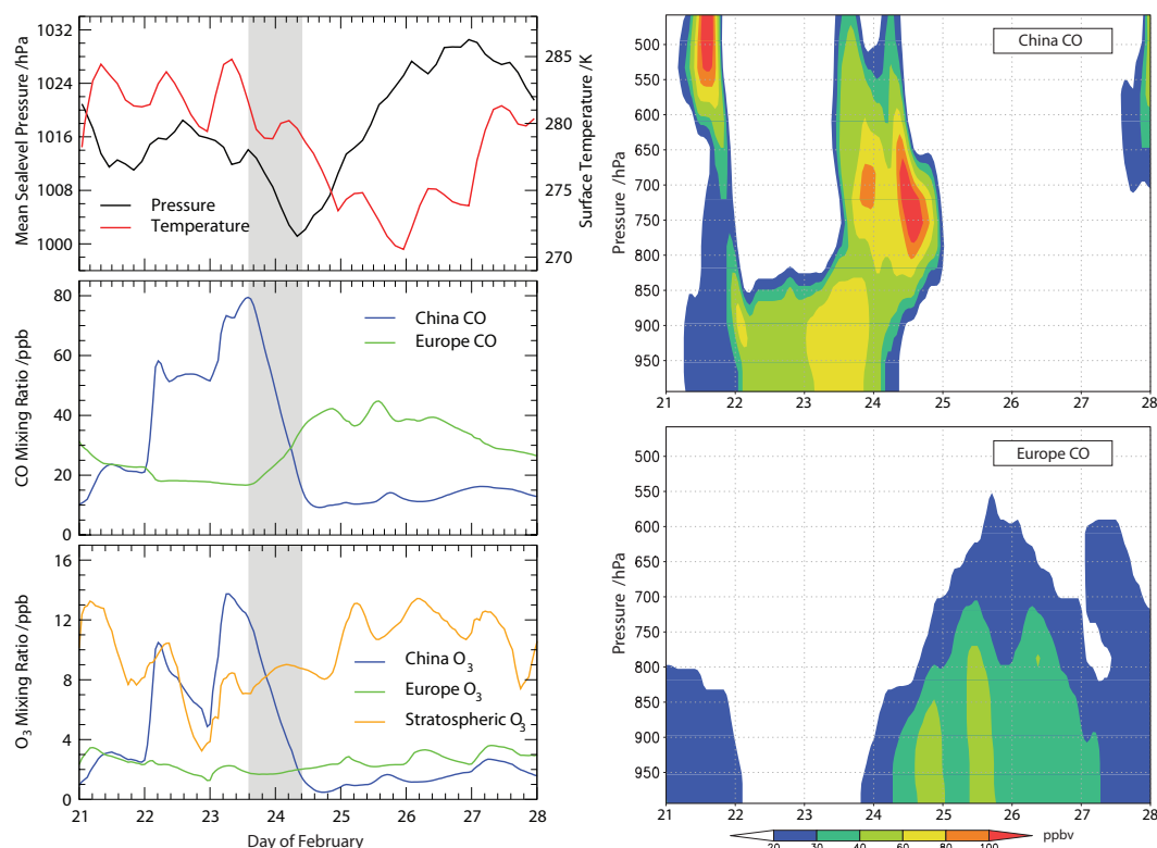
Fig. 13. Variations in surface pressure and temperature over Tokyo during the week of 21–28 February 2001, showing the passage of the frontal system shown in Fig. 12 (highlighted in grey) and the associated changes in the contribution of distant sources to \text{O}_3 and CO (left panels). Vertical profiles of the contributions of China and Europe to CO over Tokyo between the surface and 500 hPa (about 5 km) are shown in the righthand panels, highlighting the passage of the cold front on 24 February and elevated levels of CO from China aloft.
