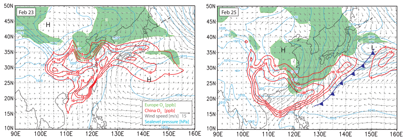
Fig. 12. Chinese and European contributions to O 3 and CO over Japan at 00:00 UTC on 23 and 25 February 2001 showing the development and movement of air masses associated with a developing frontal system (approximate position on 25 February marked in blue).
