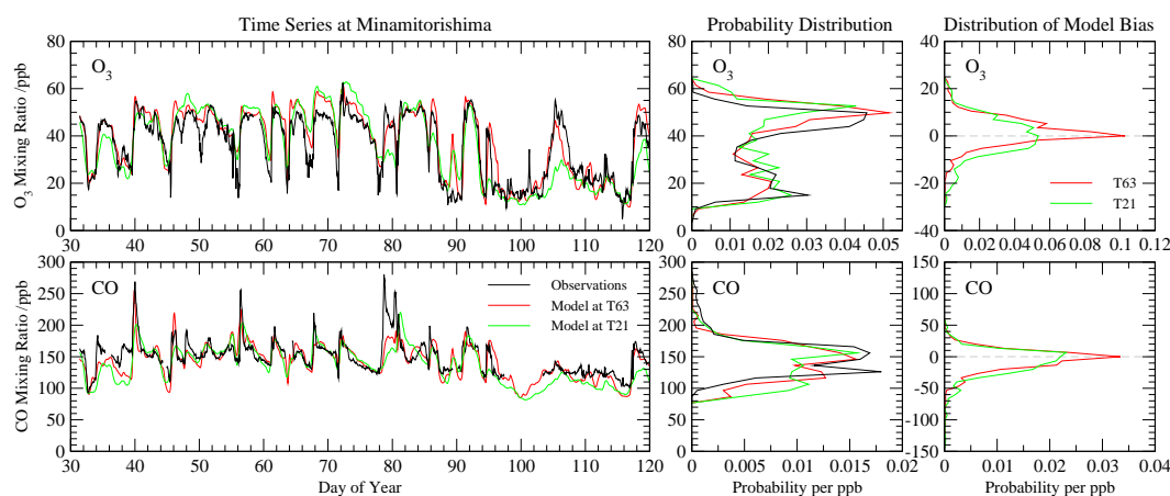
Fig. 2. Timeseries of hourly-mean surface O_3 and CO observations at Minamitorishima WMO/GAW station in February–April 2001 and FRSGC/UCI CTM results at T21 and T63 resolution. Right-hand panels show the probability distribution over the period and the distribution of the hourly model bias at each resolution.
