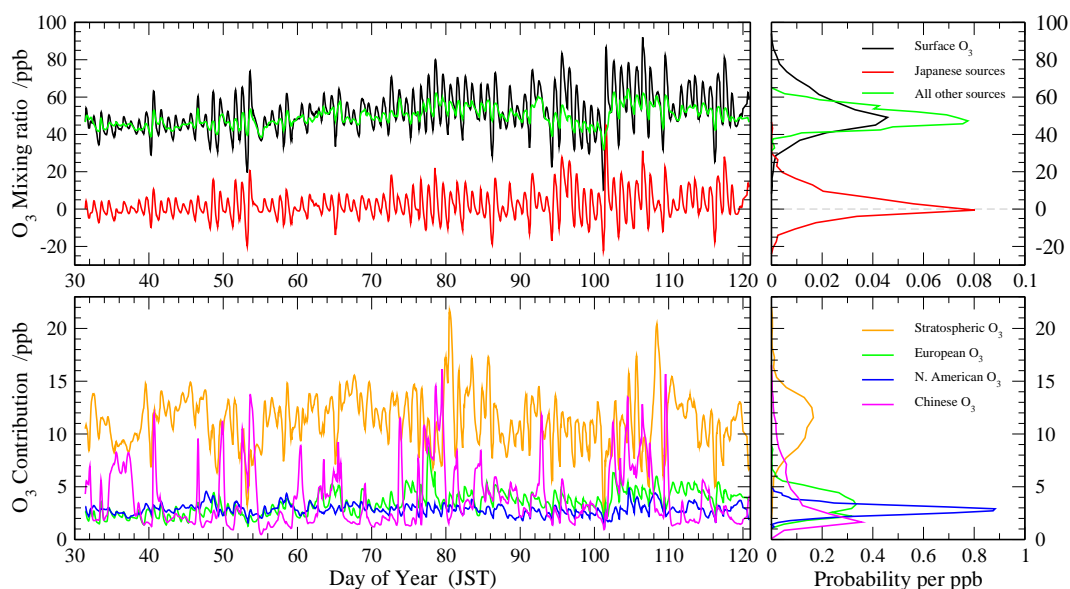
Fig. 6. Hourly mean surface \text{O}_3 mixing ratios in Tokyo in February–April 2001 from the FRSGC/UCI CTM showing (a) total surface \text{O}_3 (black), \text{O}_3 from Japanese sources (red) and the difference between them (representing \text{O}_3 from all other sources; green), and (b) contributions to \text{O}_3 from Chinese (magenta), European (green) and North American (blue) sources and from the stratosphere (orange). Right-hand panels show the probability distribution over the three-month period.
