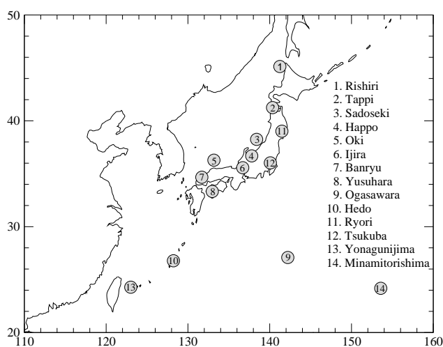
Fig. 1. Locations of EANET and WMO/GAW stations used in evaluating model performance.
