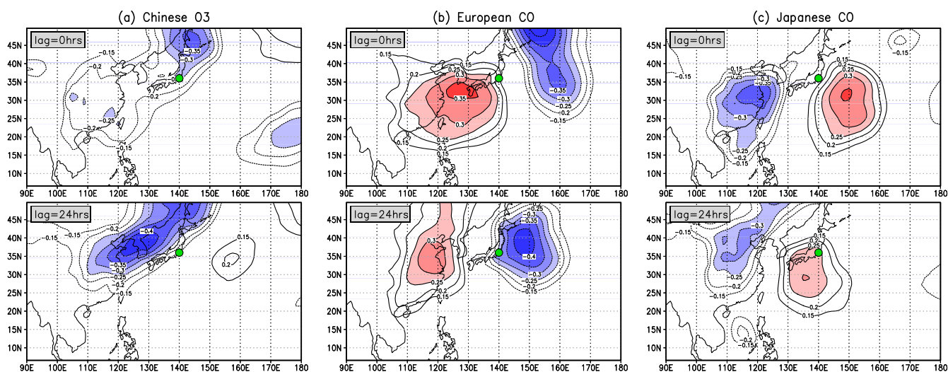
Fig. 11. Correlation between mean sea-level pressure and the contributions of (a) Chinese O 3 , (b) European CO and (c) Japanese CO over Tokyo (marked with a circle) in spring 2001. Positive correlations are highlighted in red and negative correlations in blue. Lower panels show the correlation coefficient lagged by 24 h, and thus the relationship with mean sea-level pressure one day earlier.
