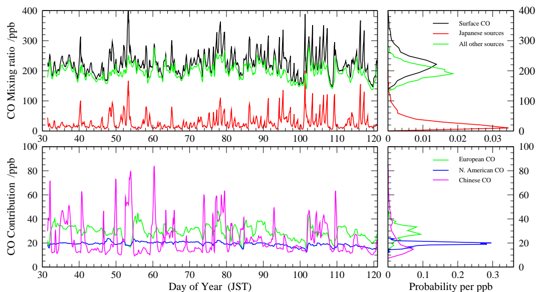
Fig. 7. Hourly mean surface CO mixing ratios in Tokyo in February–April 2001 from the FRSGC/UCI CTM showing (a) total surface CO (black), CO from Japanese sources (red) and background CO from other sources (green), and (b) contributions to CO from Chinese (magenta), European (green), and North American (blue) sources. Right-hand panels show the probability distribution over the three-month period.
