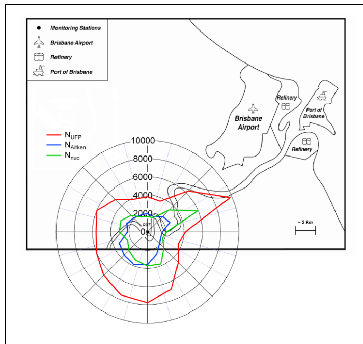
6 Figure S1: Wind rose plot of N_{\text{UFP}} , N_{\text{Aitken}} and N_{\text{nuc}} superimposed over the location map. The 7 origin of the wind rose is located at QUT. N_{\text{UFP}} - red line; N_{\text{Aitken}} - blue line; N_{\text{nuc}} - green line. 8 Unit in \text{cm}^{-3} .
