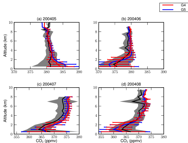
Fig. 6. Observed and GEOS-Chem a posteriori model CO 2 vertical profiles (ppm) taken from the CO 2 Budget and Regional Airborne Study over the eastern North America averaged over (a) May, (b) June, (c) July, and (d) August 2004. The GEOS-Chem model, described at a horizontal resolution of 2° × 2.5°, has been sampled at the time and location of each measurement. Data and model concentrations have been averaged over 500 m intervals. Monthly mean observations are denoted by the black lines, with the grey envelope representing the 1-standard deviation about that mean. Blue and red lines denote the monthly mean CO 2 concentrations corresponding to the G4 and G5 a posteriori flux estimates, respectively. The horizontal lines about a posteriori concentrations denote the 1-standard deviation about the monthly mean.
