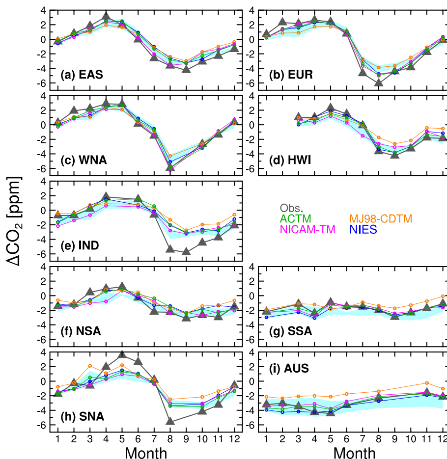
Fig. 6. Monthly mean variations of \Delta\text{CO}_2 at 5–6 km over each area for 2006–2007. Gray triangles with lines show the values for the CONTRAIL measurements. Circles with lines are for simulated results from Flux2: ACTM (green), MJ98-CDTM (orange), NICAM-TM (magenta), and NIES (blue). Cyan shade shows range of the simulated results from Flux1.
