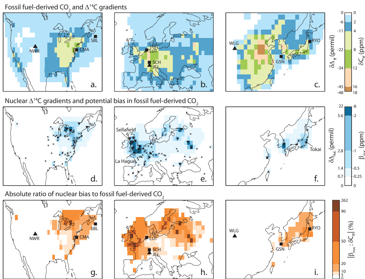
Fig. 2. (a–c) Maps of fossil fuel-derived \text{CO}_2 ( \delta C_{\text{ff}} ) and \Delta^{14}\text{C} dilution ( \delta\Delta_{\text{ff}} ) in continental regions of the Northern Hemisphere. Regional reference sites are indicated by triangles and observation sites by squares. (d–f) Nuclear \Delta^{14}\text{C} enhancement ( \delta\Delta_{\text{nuc}} ) and potential nuclear bias to fossil fuel-derived \text{CO}_2 ( \beta_{\text{nuc}} ). Locations of low- ^{14}\text{C} release reactors are indicated by crosses, high- ^{14}\text{C} release reactors by triangles, and spent fuel reprocessing sites are labeled. (g–i) The ratio |\beta_{\text{nuc}} : \delta C_{\text{ff}}| , in percent, shown only in grid cells where \beta_{\text{nuc}} was less than -0.25 ppm.
