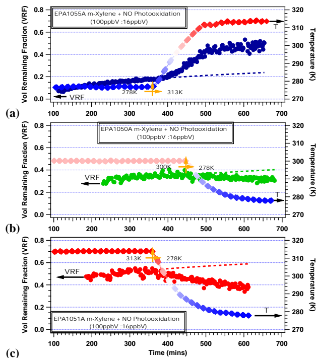
Fig. 4. The volume remaining fraction in typical operating schemes for m -xylene photooxidation experiment at three temperatures (a) 278 K → 313 K; (b) 300 K → 278 K; (c) 313 K → 278 K.
